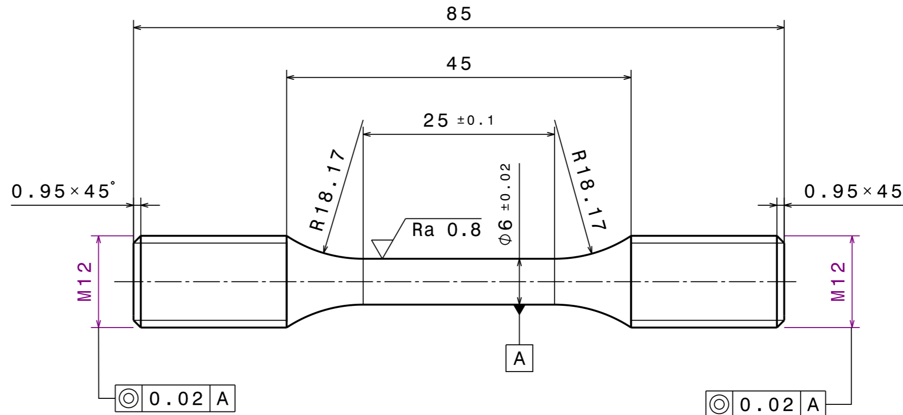
SIDE VIEW SCALE 2:1
