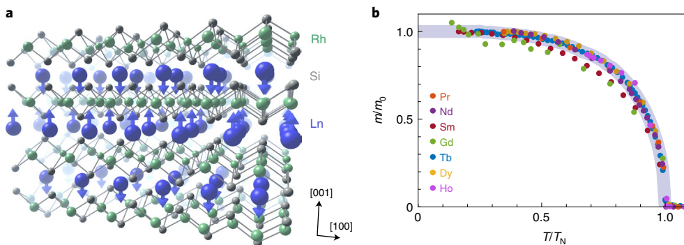
Fig. 1 | The \text{LnRh}_2\text{Si}_2 materials. a , The layered crystal structure, highlighting the layer-by-layer antiferromagnetic reversal along the [001] direction (for \text{Ln} = \text{Sm} and \text{Gd} , moments lie in-plane). b , Temperature dependence of the \text{Ln}^{3+} sites' ordered 4f moment in all materials, exhibiting mean-field-like behaviour. The axes are normalized by each material's saturated moment m_0 and Néel temperature T_N . The data were extracted from temperature-dependent resonant magnetic X-ray diffraction experiments (Methods). The grey line is a guide for the eye representing mean-field behaviour.
