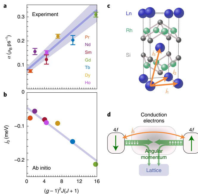
Fig. 3 | De Gennes scaling and RKKY coupling. a , Experimental values of the maximal angular momentum transfer rates (explanation in main text) as a function of the de Gennes factor G . Data are shown for F/F_C = 0.37 (other fluences behave very similarly). The best fit to a linear trend is presented, with a shaded area representing the error margin (slope: (15 \pm 2)10^{-3} \mu_B \text{ps}^{-1} ; offset: (78 \pm 14)10^{-3} \mu_B \text{ps}^{-1} ). b , Calculated RKKY coupling between the nearest antiferromagnetically aligned Ln ions, also plotted against G . The line is a guide for the eye. c , Sketch of an extended unit cell with the nearest RKKY couplings indicated; j_3 is the interlayer coupling. d , Diagram depicting the flow of 4f angular momentum after excitation, in which conduction electrons mediate the flow between 4f states on antiparallel sites, as well as the flow to the lattice. Errors are defined in the Methods section.
