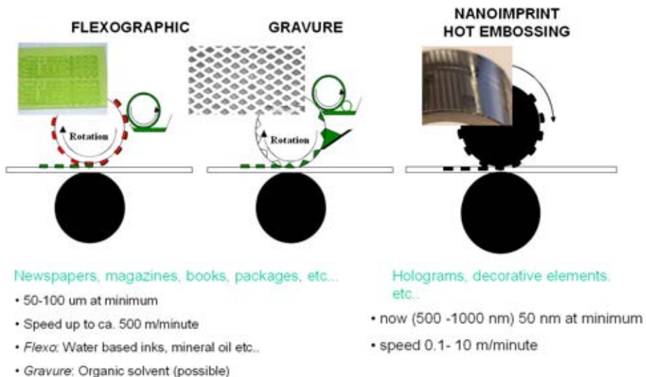
Figure 5.27: Schematic of different roll-to-roll processes.
