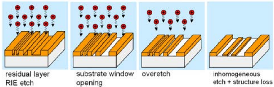
Figure 5.33: Process sequence for residual layer etching.
