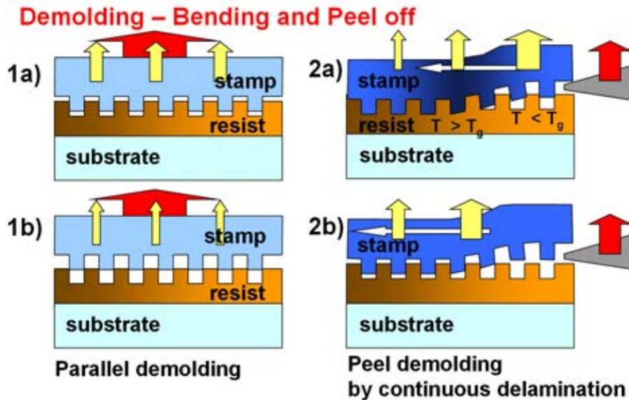
Figure 5.32: Principle for parallel and wedge induced demolding.
