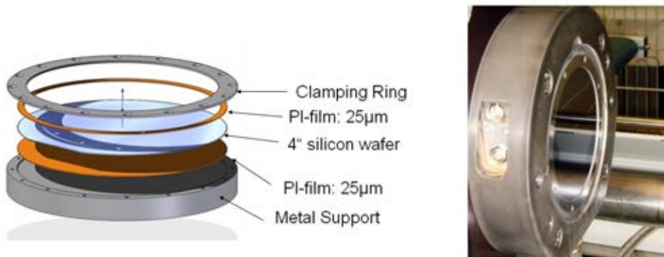
Figure 5.29: Left side: Clamping system for a 4" wafer used as insert for injection molding. Right side: Tool with ejection side of the injection mold with structured 4" silicon wafer.
