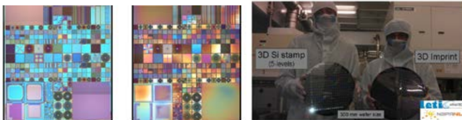
Figure 5.9: Multilevel stamp fabrication using DUV- projection lithography. Depending on the arrangement of the layers, different strategies for pattern transfer need to be applied.
