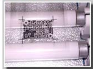
+ Exposure setup
