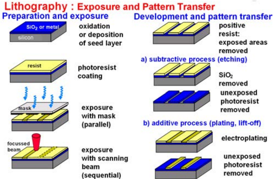
Figure 4.3: Example of standard photon and electron based lithography and pattern transfer.
