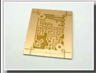
Developed Resist
