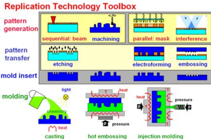
Figure 5.6: Process toolbox that summarizes a range of process variants from origination and tooling to molding.
