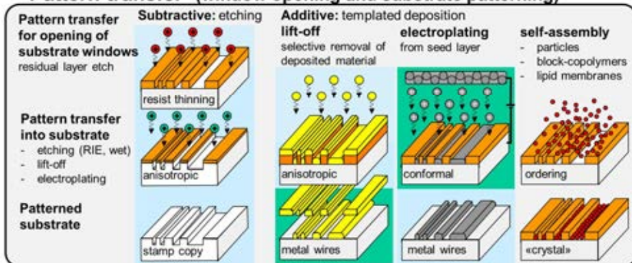
Figure 3.1: Nanoimprint lithography (NIL) consists of the three major steps origination, replication and pattern transfer.
