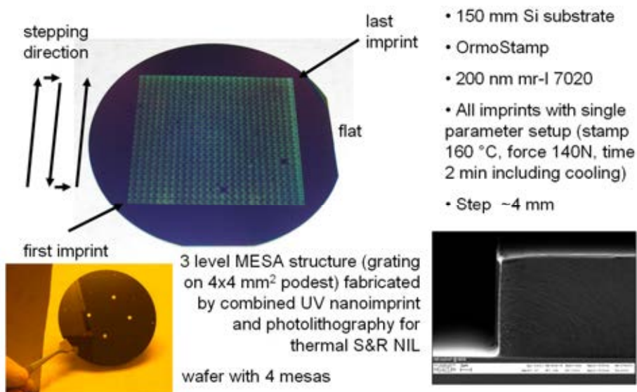
Figure 5.13: Large area S&R thermal NIL with OrmoStamp ® copy: In order to create a 4x4 mm 2 mesa on a base of a 10x10 mm 2 large stamp (to decouple the active area from the heated base), the imprint into the OrmoStamp ® layer was combined with a masked exposure of the 4x4 mm 2 wide mesa. Afterwards the non-crosslinked material was dissolved.
