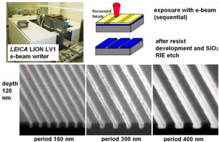
Figure 5.7: Exposure and pattern transfer for stamp fabrication by electron beam lithography and reactive ion etching.
