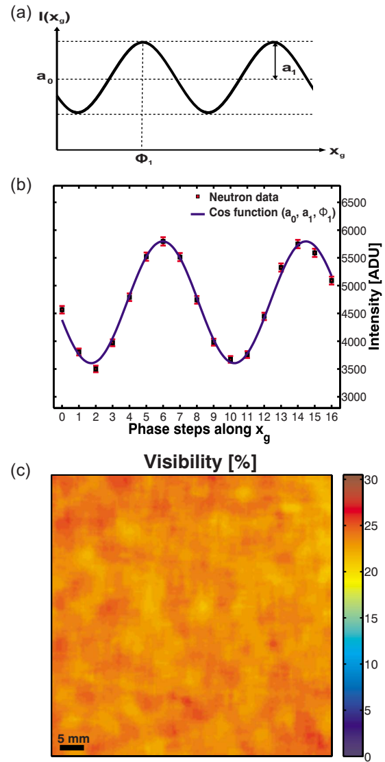
FIG. 5. (Color online) Characterization of the gratings. (a) Depiction of the intensity modulation for one detector pixel when one of the gratings is scanned along x_g and the corresponding Fourier series coefficients a_0 , a_1 , and \phi_1 (see text). (b) Neutron data of the intensity modulation for a single detector pixel and the corresponding cosine function obtained from the extracted Fourier coefficients. (c) Visibility map over the whole grating area of 64 \times 64\ \text{mm}^2 showing the values of a_1/a_0 for each detector pixel with an averaged value of 23%.
